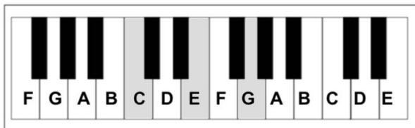
C Major: C-E-G
