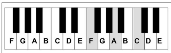
F Major: F-A-C
