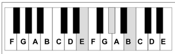
E Major: E-G#-B
