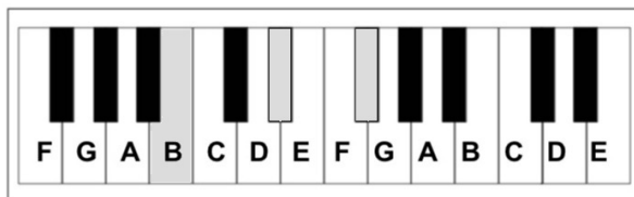
B Major: B-D#-F#
